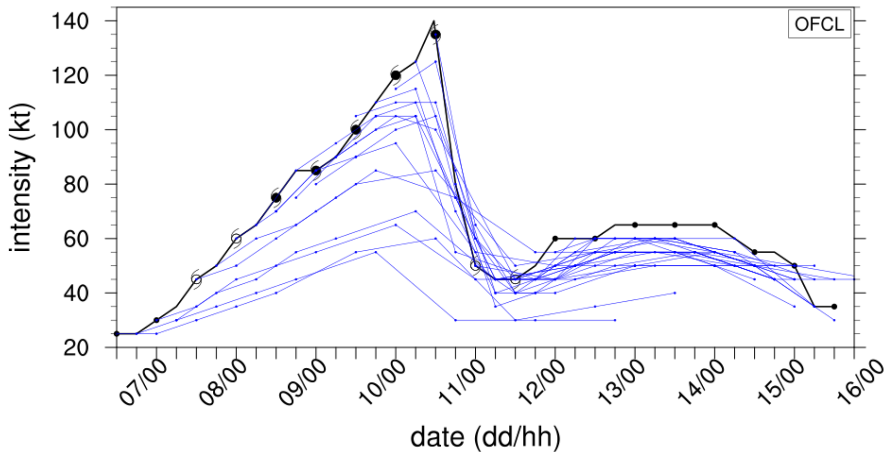
Figure 12. Selected NHC official intensity forecasts (kt, blue lines) for Hurricane Michael. The best track intensity (kt) is given by the black line with the symbols at 6 h intervals.
