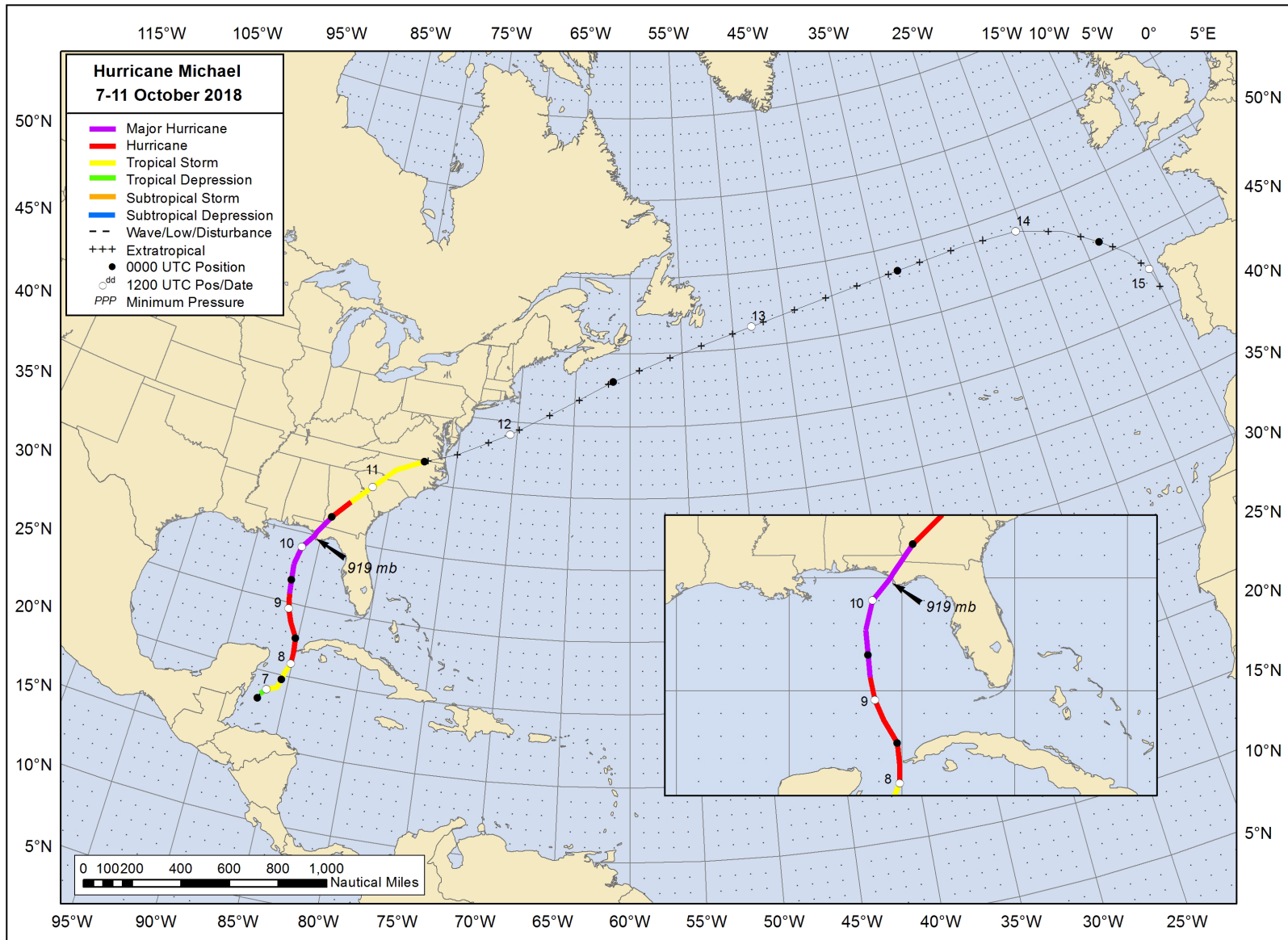
Figure 1. Best track positions for Hurricane Michael, 7–11 October 2018. The track during the extratropical stage is partially based on analyses from the NOAA Ocean Prediction Center.
